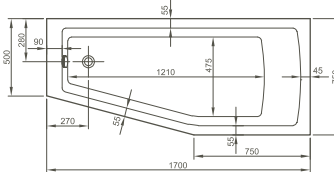
Raumsparwanne, Ecke links/Spacesaving Bathtub, corner left
